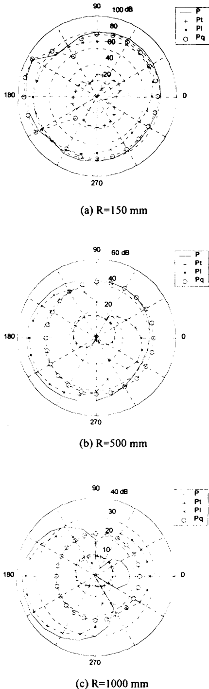
Fig. 6 Noise directivity of each noise term (3600rpm, Re = 9 \times 10^4 )
