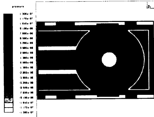
Fig. 3 Contour of pressure distribution at low surface of disk; CFD result at angular velocity 7200 rpm (unit: GPa)
