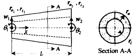
Fig. 3 Beam element with varying section
