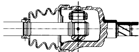
(c) Tri-pot joint
