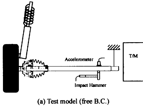
(a) Test model (free B.C.)
