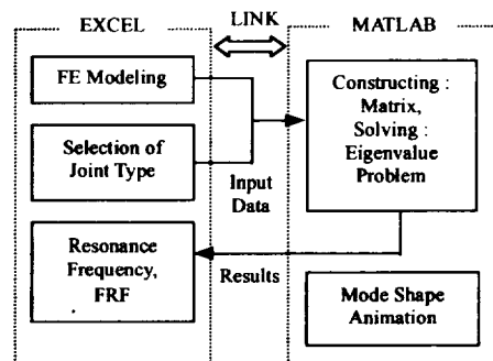
Fig. 7 Structure of simulation program
