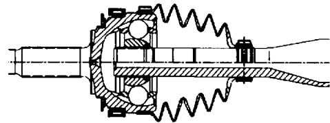
(a) Rzeppa joint
