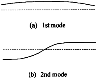
Fig. 5 Mode shapes of drive shaft by modal test
