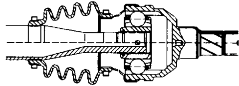
(b) Cross-groove joint
