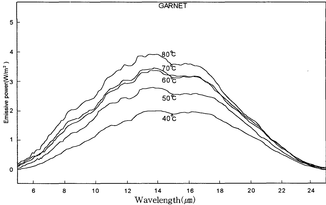
Fig. 3. Emissive power of garnet at different temperatures.
