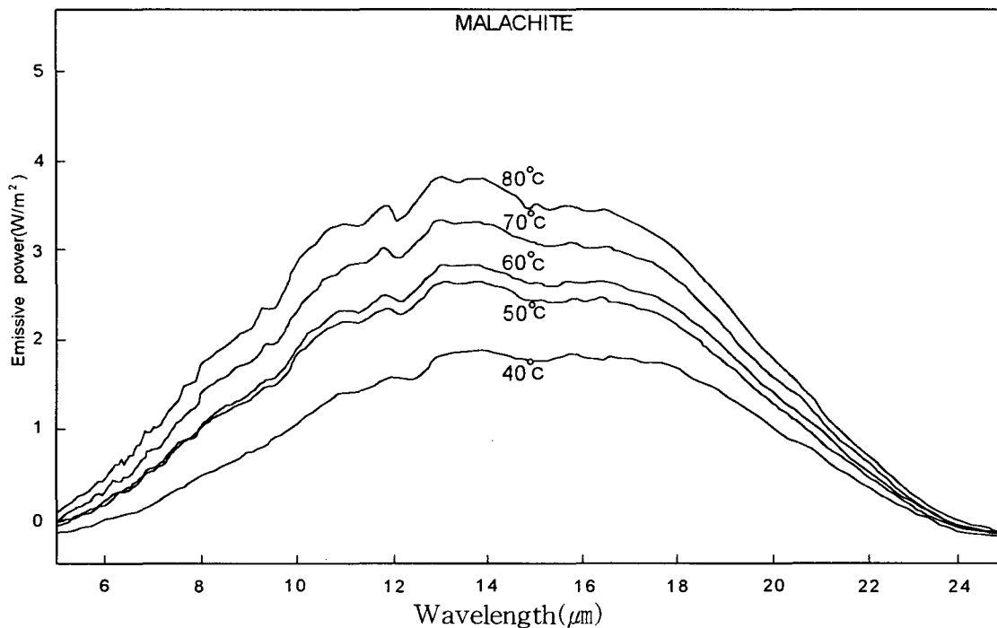
Fig. 2. Emissive power of malachite at different temperatures.
