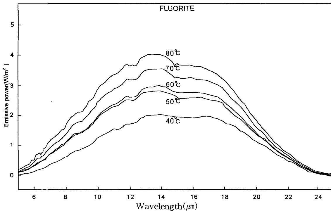
Fig. 1. Emissive power of fluorite at different temperatures.
