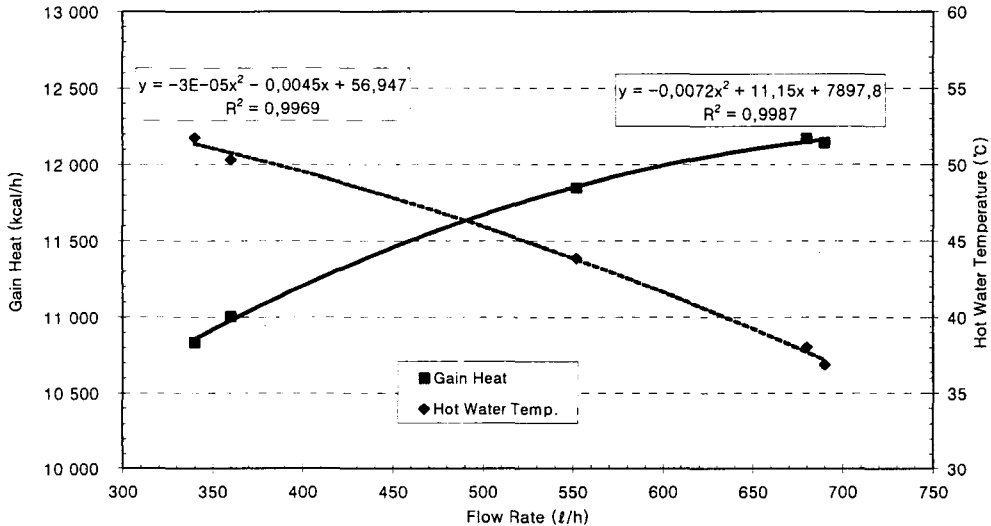
Figure 4. Relationship between heat exchange amounts and hot water temperatures in the heater exchanger used in this experiment
