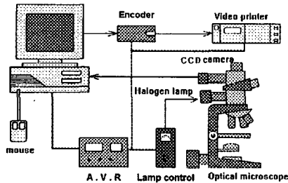
Fig. 4 Schematic diagram of image processing system
