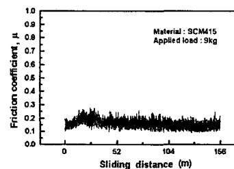
Fig. 6 Relation between friction coefficient and sliding distance.
