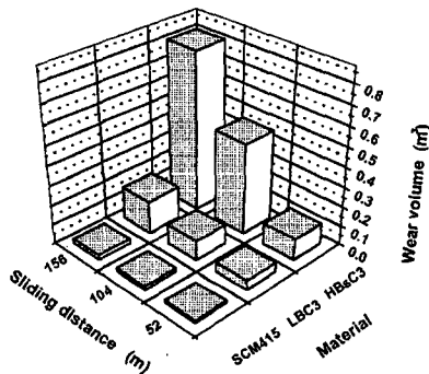
Fig. 11 Wear volumes for specimen
