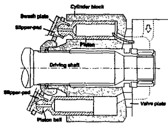
Fig. 1 Hydraulic piston motor
