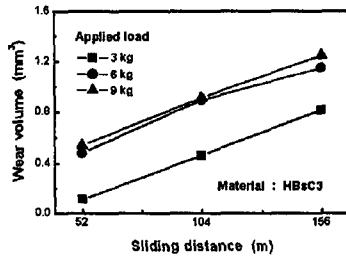
Fig. 10 Effect of applied load on wear volume
