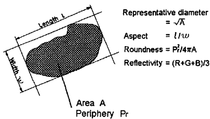
Fig. 5 Shape parameters of wear particle
