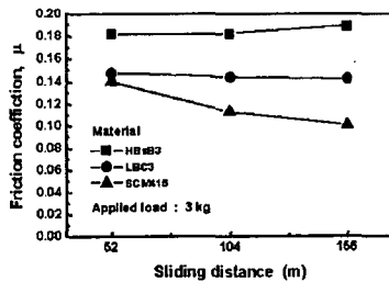
Fig. 7 Friction coefficient for specimen
