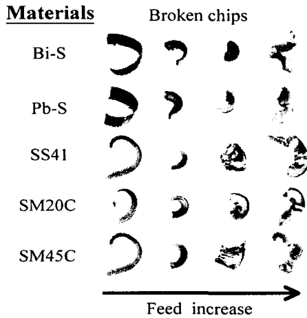
Fig. 4 Types of broken chips.
