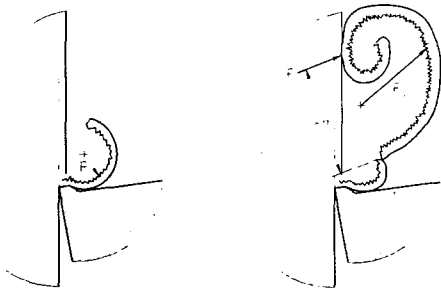
(a) Before chip breaking (b) After chip breaking
