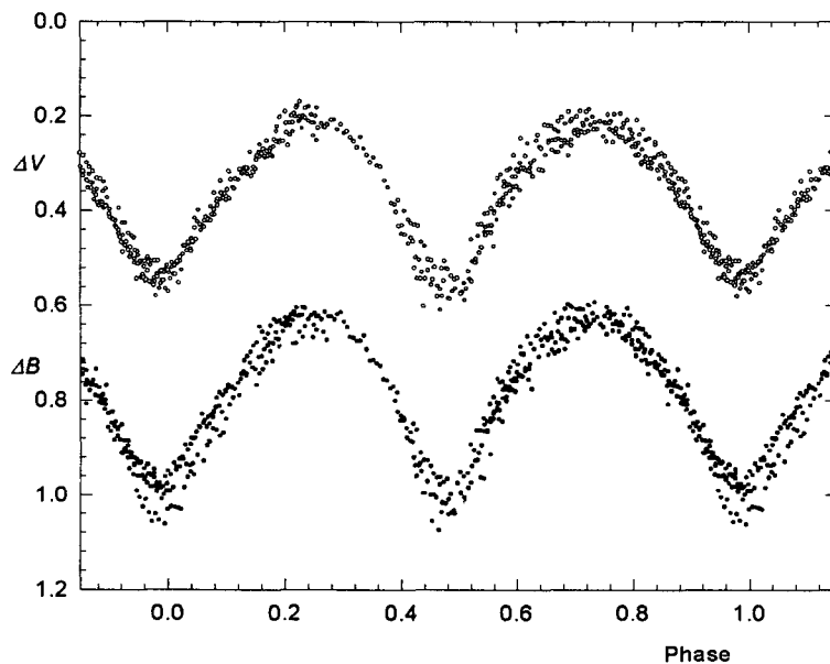
Figure 1. BV light curves of VW Cep.
