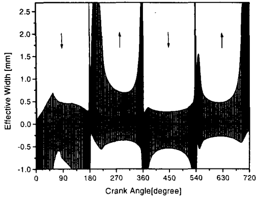
Fig. 4 Effective width of piston ring
