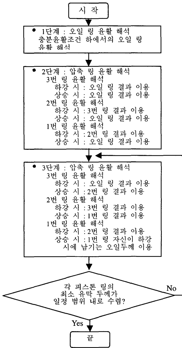
Fig. 8 Flow Chart for Ring Pack Analysis
