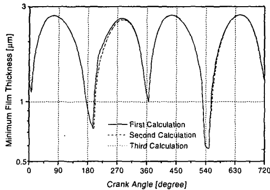
Fig. 12 Minimum film thickness between the Third Ring and Cylinder Liner according to Analysis Sequence
