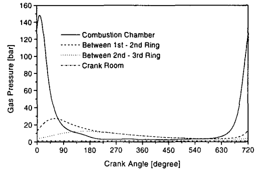
Fig. 5 Inter-ring Gas Pressure
