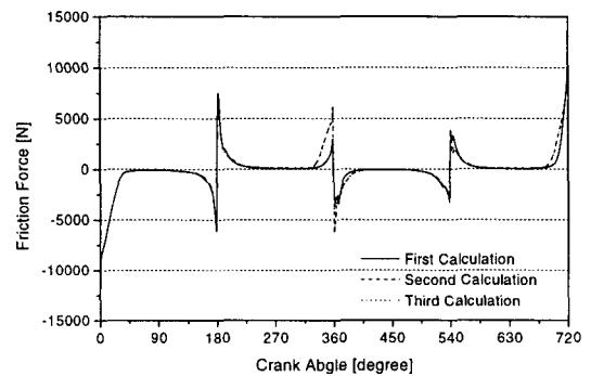
Fig. 10 Friction force on the Top Ring according to Analysis Sequence
