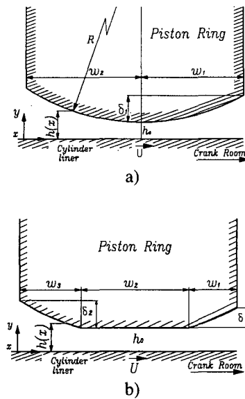
Fig. 6 Surface Shape of the Compression Ring
