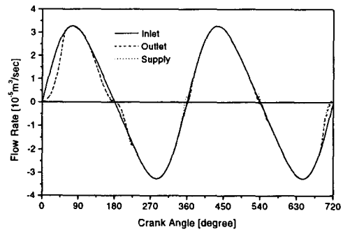
Fig. 3 Flow quantity at the inlet and outlet
