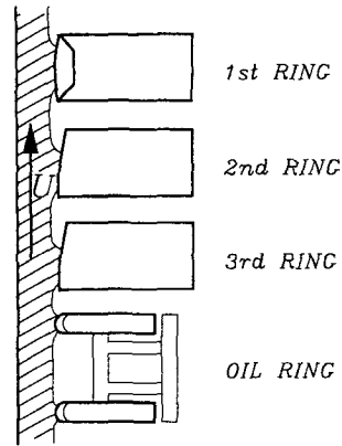
Fig. 7 Oil Flows in the Ring Pack
