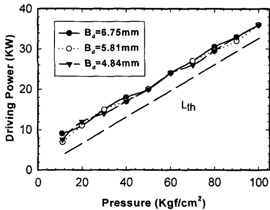
Fig. 10 Effect of change of B_d with driving power
