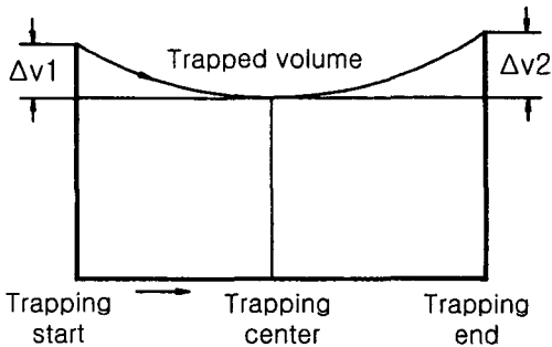
Fig. 2 Variation of the trapped volume
