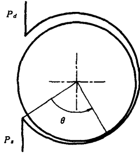
Fig. 7 The site of minimum tip clearance
