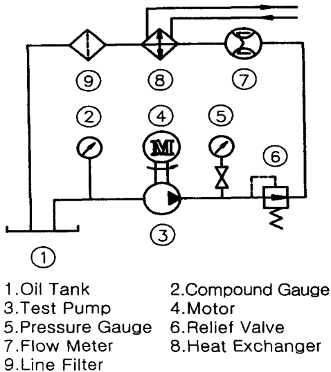
Fig. 6 Circuit of oil hydraulics
