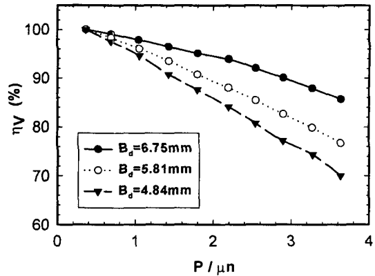
Fig. 11 Variation of volumetric efficiency according to change of B_d
