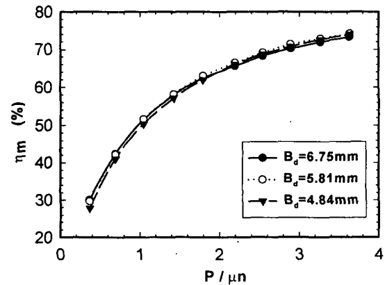
Fig. 12 Variation of mechanical efficiency according to change of B_d
