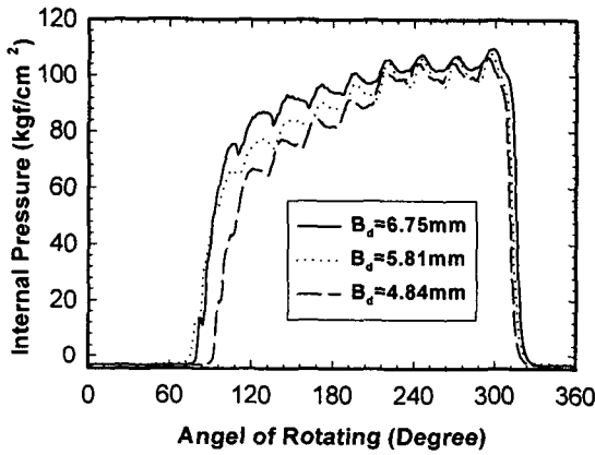
Fig. 8 Variation of internal pressure distribution according to change of B_d
