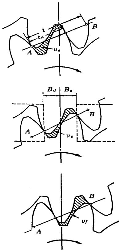
Fig. 1 Trapping with gears
