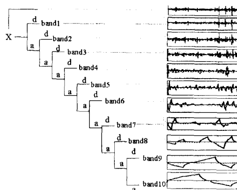
Figure 7. Tree algorithm using daily Korean Won / US Dollar returns (X: original series, a: approximation components, d: detailed components, band 1 (the highest highpass filter) → band10 (the lowest lowpass filter))
