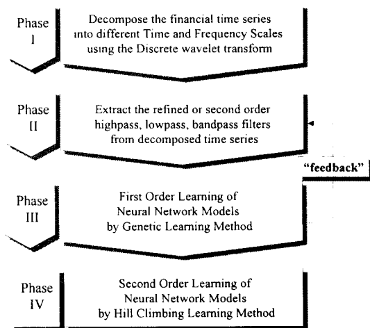
Figure 5. Proposed Research Framework
