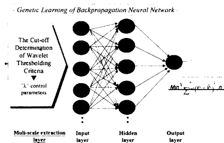
Figure 6. A Hybrid Neural network Model Architecture
