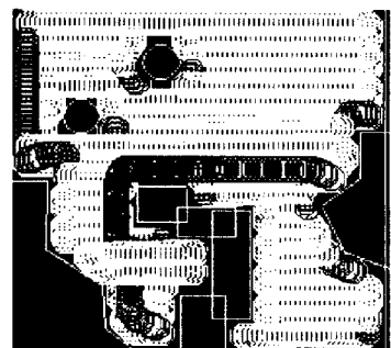
Fig. 5 Final resultant sweeping path (with collision avoidance)
