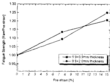
Fig. 7 Fatigue resistance of pre-strained specimen
