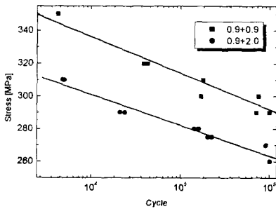
Fig. 4 Fatigue test results of laser weld (0.9+0.9, 0.9+2.0 thickness, longitudinal direction)
