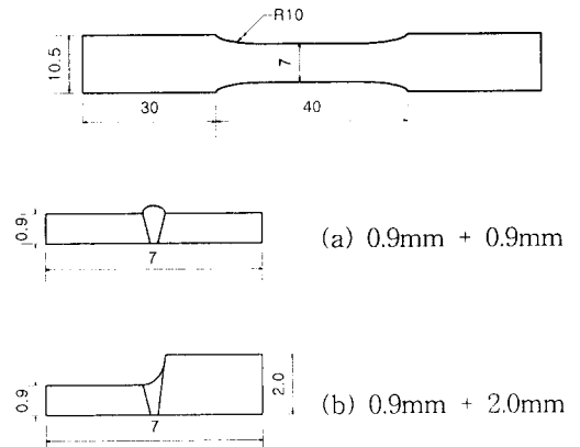
Fig. 1 Dimension of Specimens for fatigue strength test
