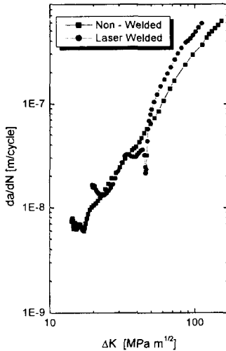
Fig. 9 Fatigue crack propagation
