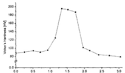
Fig. 3 Micro Vicker's Hardness
