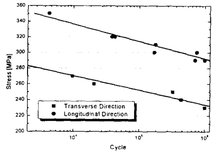
Fig. 5 Fatigue test results of laser weld (0.9+0.9 thickness, transverse, longitudinal direction)
