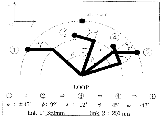
Fig. 13. Kinematic configuration of repeating precision.
