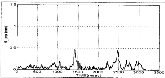
Fig. 10. Tracking error of neural controller with 2.0 kg payload.
