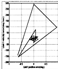
Fig. 6. Performance analysis at error state space.
