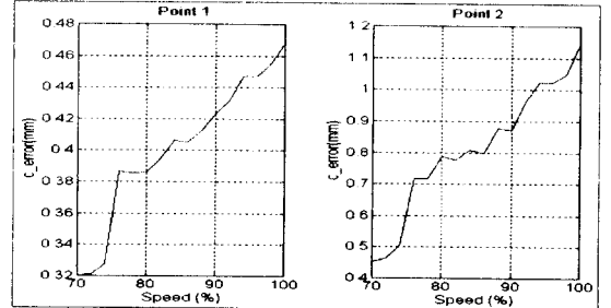
Fig. 14. Experimental results of neural controller for repeating precision at cartesian coordinates.
