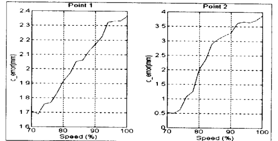
Fig. 15. Experimental results of existing controller (PID) for repeating precision at cartesian coordinates.
