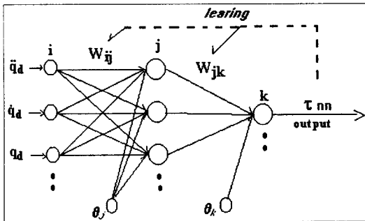
Fig. 1. Neural Network Structure
