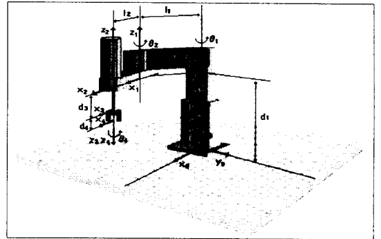
Fig. 3. Coordinates frame of SCARA robot.
