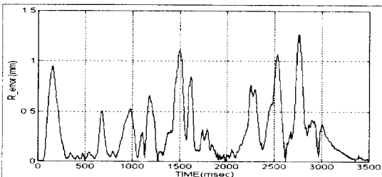
Fig. 12. Tracking error of existing controller(PID) with 2.0 kg payload.
