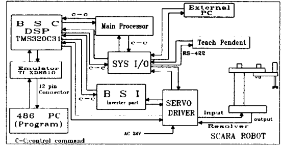
Fig. 7. The block diagram of control system.
