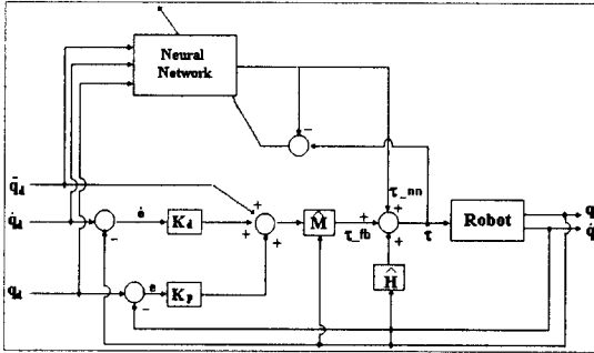
Fig. 2 The block diagram of proposed neural control Structure for robot manipulator
