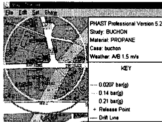
Fig. 2-4. Effect distance by LPG Overpressure
