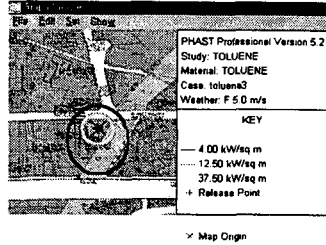
Fig. 2-1. Radiation effect of Toluene, wind speed 5.0m/s, hole size 100mm
