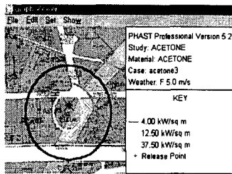
Fig. 2-3. Radiation effect of Acetone, wind speed 5.0m/s, hole size 100mm
