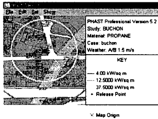
Fig. 2-5. Radiation Heat of Fireball
