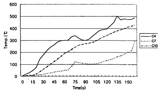
그림 4. Different variation of temperature profile in the fire room between on the middle part of window glass and on the window glass inside the flame (in the test 1-3) (C4:upper point of inside, C7:upper point of outside, C10:Inside point of frame )
