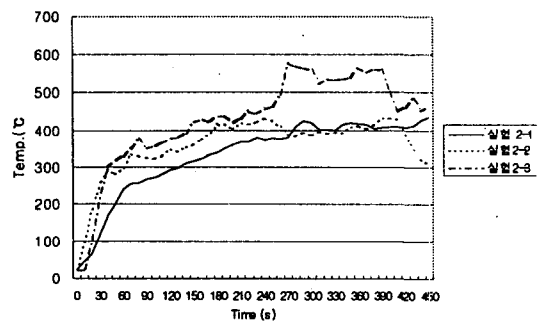
그림 5. Variation of temperature profile. Outside window glass of the upper part (in the test 1-2, 2-2, 2-3)
