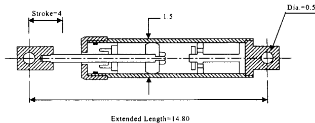
Figure 3 Hydraulic Damper
