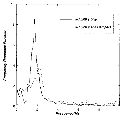
Figure 4 Frequency Response Functions for Deck Acceleration of Isolated Bridges from the Test Results Using White Noise Excitation
