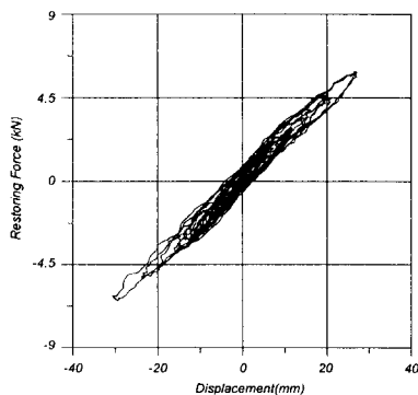
(a) Isolated w/ LRB's only
