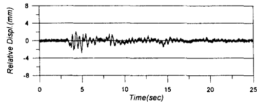
(b) Isolated w/ LRB's and Dampers
