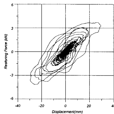
(b) Isolated w/ LRB's and Dampers
