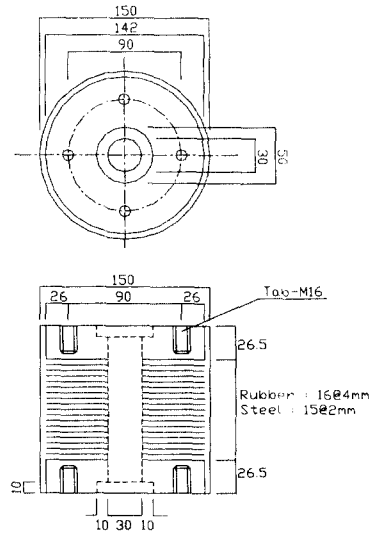
Figure 2 Dimension of Natural Rubber
