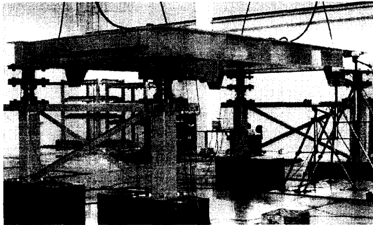
(a) Overview of Test Structure
