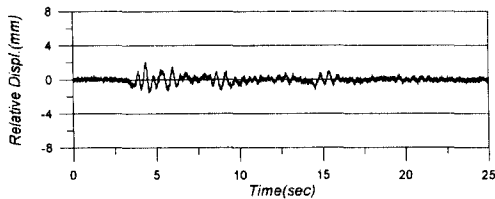
(a) Isolated w/ LRB's only
