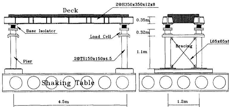
(b) Dimensions of Test Structure
