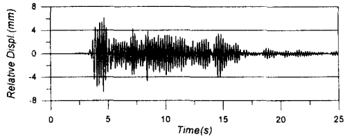
(a) Un-Isolated Bridge
