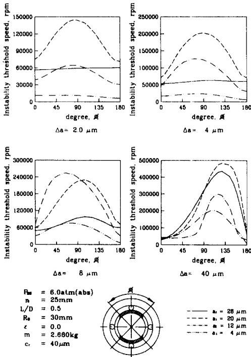
Fig. 6 Instability threshold speed of non-circular slot
