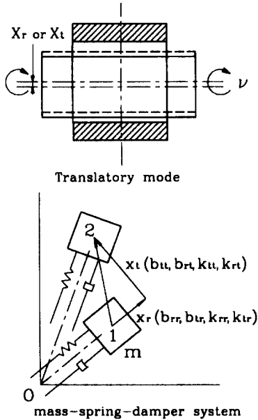
Fig. 3 Vibration mode of journal and equivalent system
