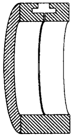
Fig. 1 Slot bearing
