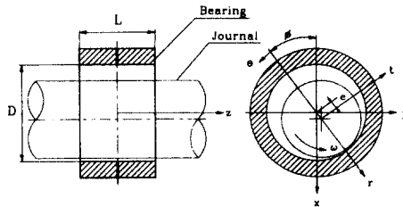
Fig. 2 Bearing coordinates system
