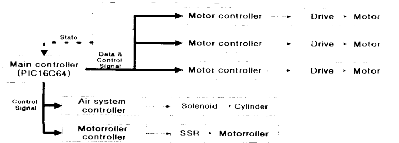
Fig 8. Organization of the system controller.
