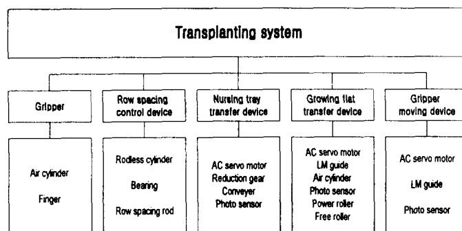
Fig 1. Schematic diagram of the robotic transplanter.
