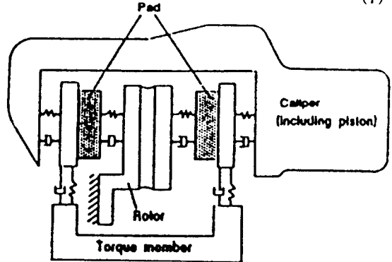
Fig.1 Schematic diagram of brake
