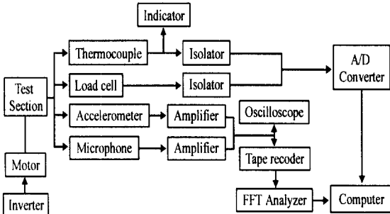
Fig.6 Schematic diagram of data acquisition
