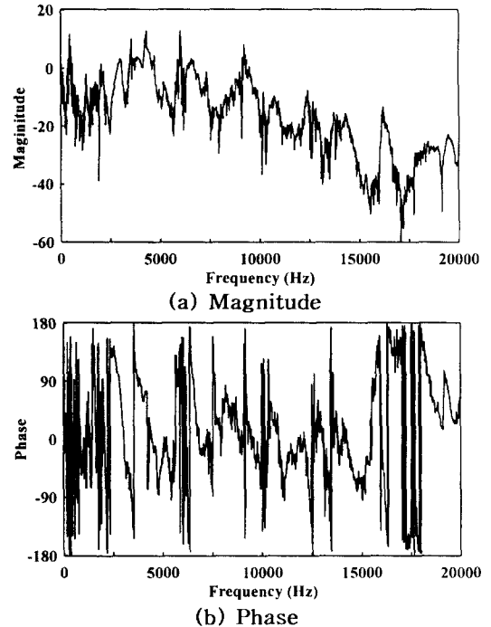
Fig.12 Frequency Response Function (between vibration and noise)
