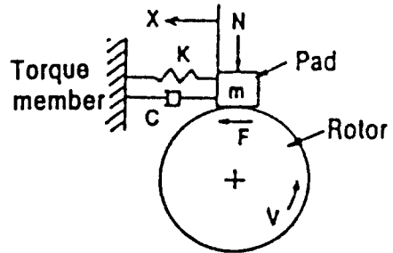
Fig.1 Schematic diagram of brake
