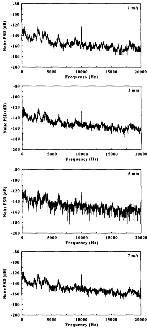
Fig.10 Comparison of noise power spectrum density with squeal
