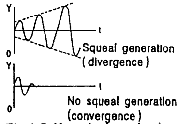
Fig.4 Self-excited mechanism with feedback system
