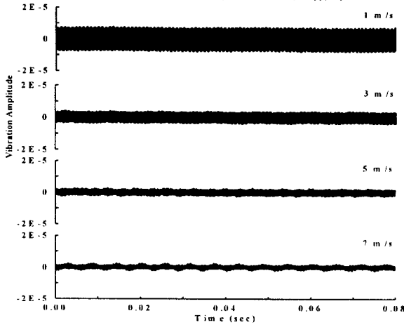
Fig.7 Comparison of brake vibration amplitude with squeal
