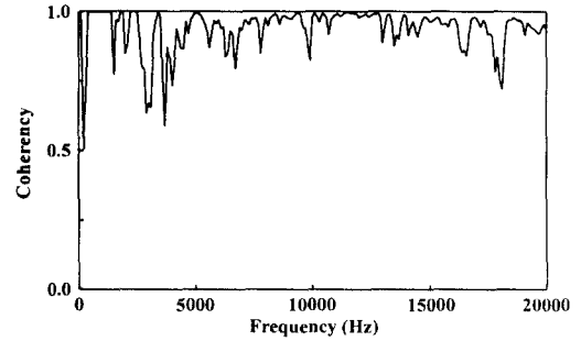
Fig.11 Coherence function
