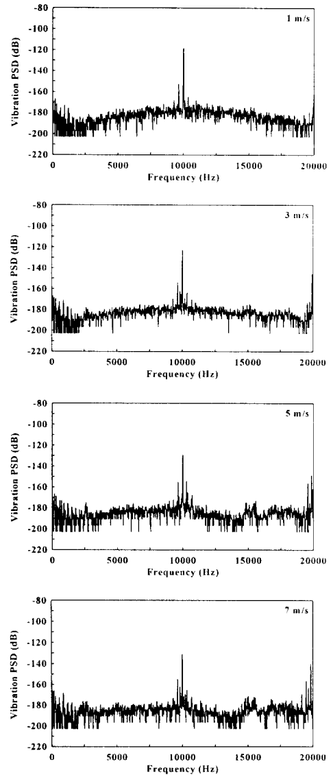
Fig.9 Comparison of vibration power spectrum density with squeal
