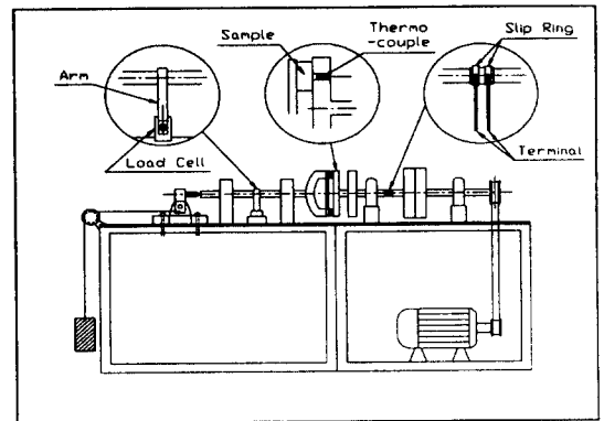
Fig.5 Schematic diagram of scale tester
