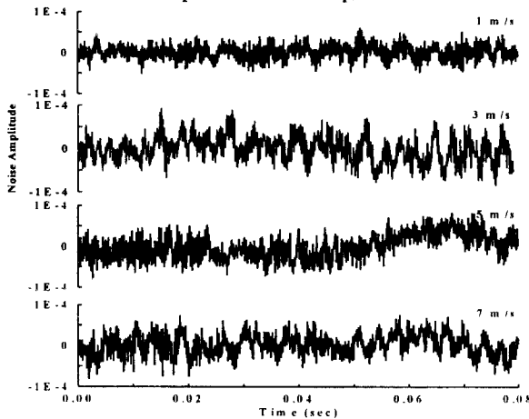
Fig.8 Comparison of brake noise amplitude with squeal
