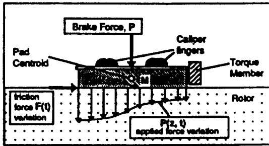
Fig.3 Axial effective brake force variation
