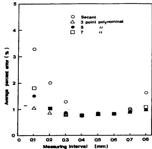
Fig. 8 Average percent error in calculating N from da/dN versus measuring intervals ( \Delta K constant test)
