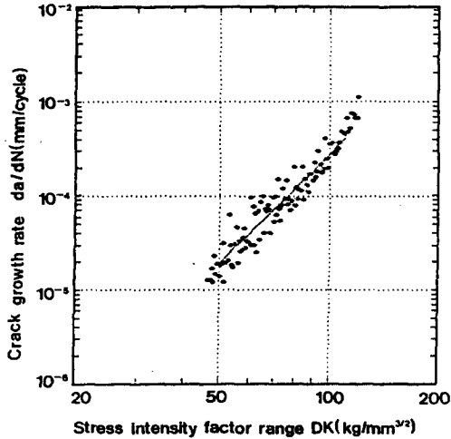
Fig. 4 Relation between stress intensity factor and crack growth rate (measuring interval : 0.1mm, da/dN calculation : secant method)
