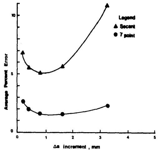
Fig. 6 Average percent error in calculating N from da/dN versus the \Delta a increment size
