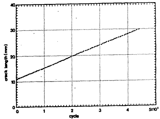
Fig. 3 Relation between crack length and cycle ( \Delta K constant test)
