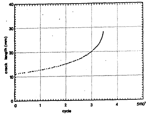
Fig. 2 Relation between crack length and cycle ( \Delta P constant test)
