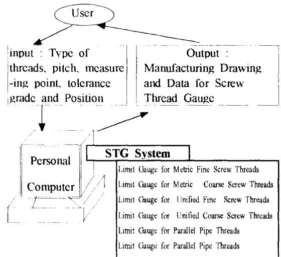
Fig 2. Concept of the Screw Thread Gauge CAD System
