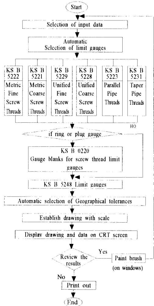
Fig 3. Structure of STG System
