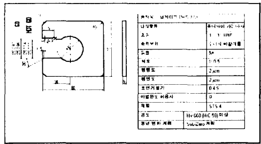
Fig. 7 Snap gauge for unified fine screw thread - major diameter
