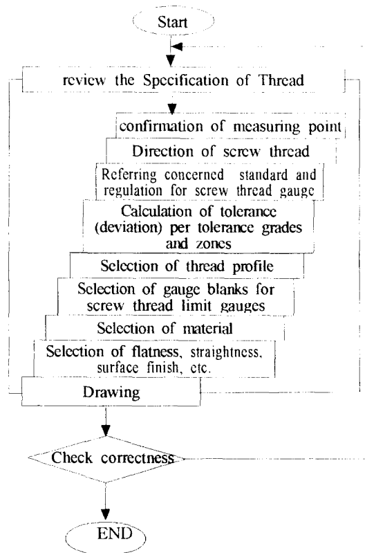
Fig. 1. Limit gauge Design and Drawing Process
