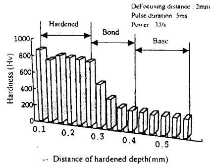
Fig. 9 Relationship between hardened depth and hardness
