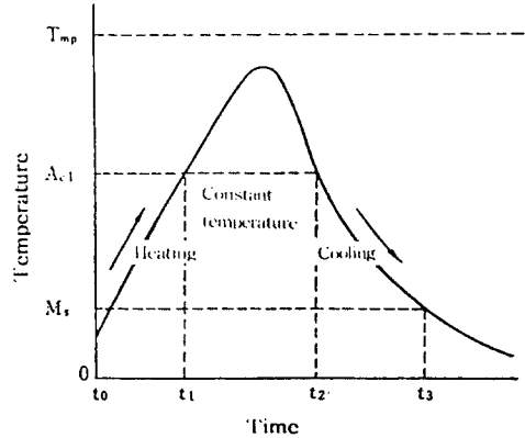
Fig. 2 Temperature curve of surface hardening process by laser beam.
