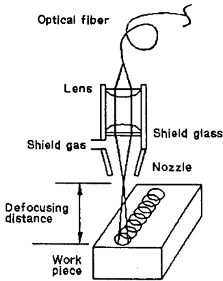
Fig. 3 Schematic view of laser irradiation
