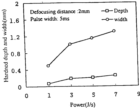
Fig. 7 Molten depth and width on laser power
