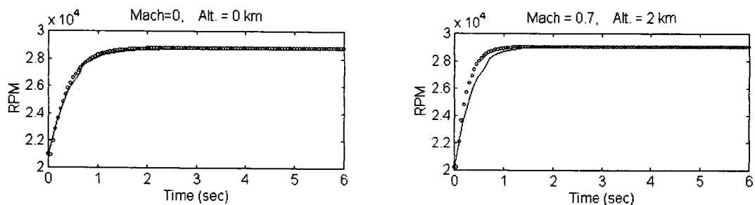
Figure 1. The Comparison of Results between Nonlinear Simulation and Real Time Linear Simulation (----- Nonlinear Simulation, ooooo Real Time Linear Simulation)
