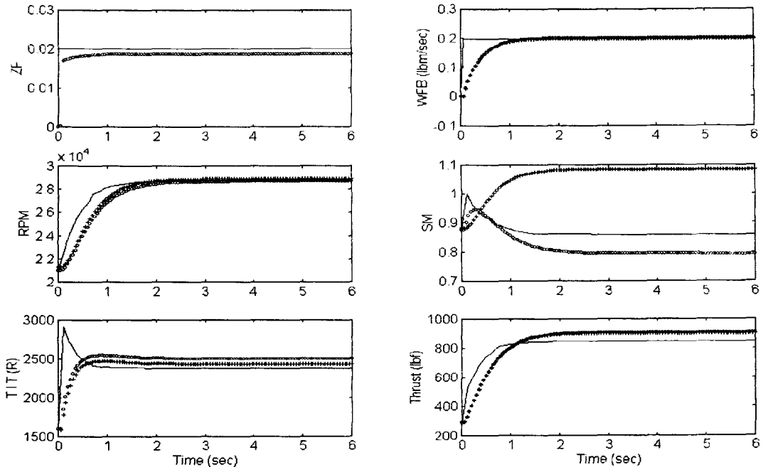
Figure 2. The Comparison of the Response with Various Model (---Nonlinear, +++LQR Control with Single Input, oooLQR Control with Multi-Input) in Case 1
