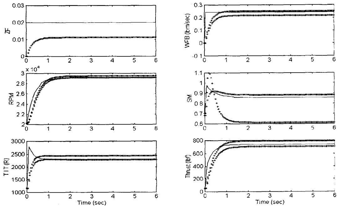
Figure 3. The Comparison of the Response with Various Model (---Nonlinear, +++LQR Control with Single Input, oooLQR Control with Multi-Input) in Case 2
