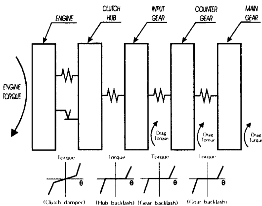
Fig. 2 Physical 5 DOF model to analyze the idle gear rattle
