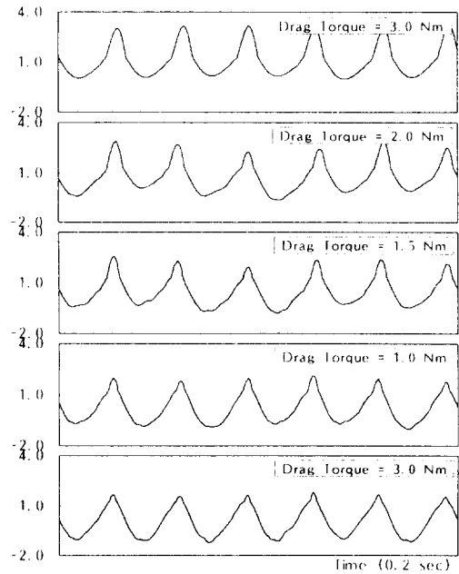
Fig. 5 Influence of drag torque on the clutch operating angle[degree]
