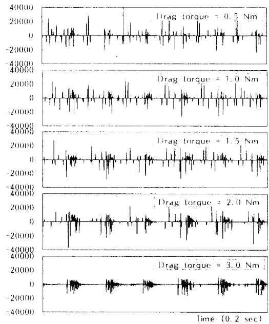
Fig. 4 Influence of drag torque (angular acceleration of input gear [rad/sec 2 ])
