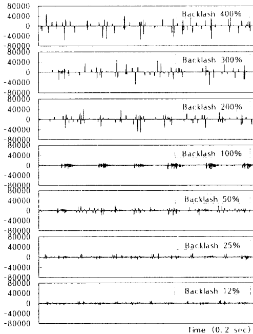
Fig. 3 Influence of backlash
