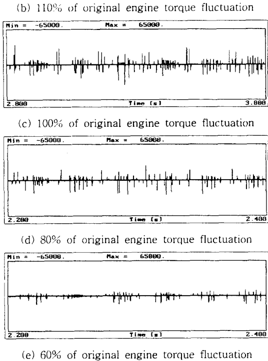
Fig. 9 Influence of engine torque fluctuation (angular acceleration of input gear [rad/sec 2 ])
