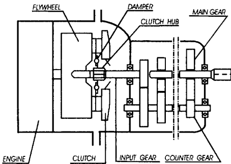
Fig. 1 Schematic diagram of manual transmission
