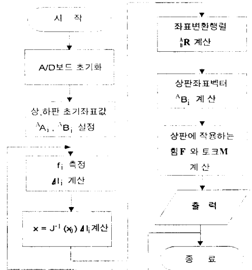
Fig. 2 The order for computing the force F and torque M acting on the upper plate from the forces acting on the six legs.
