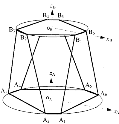
Fig. 1 Kinematic structure of Stewart platform and body-attached coordinate frames
