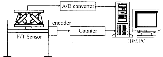
Fig. 4 The schematic diagram of a experiment system
