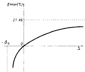
Fig. 5 Error vs. the distance between the centers of the shaft and the lip seal
