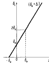
Fig. 4 Interference as a function of the distance between the centers of the shaft and the lip seal
