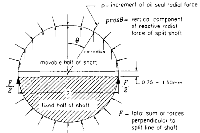
Fig. 2 Principle of a split shaft device
