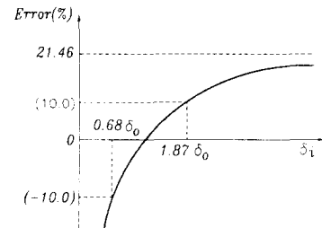
Fig. 7 Error as a function of interference.
