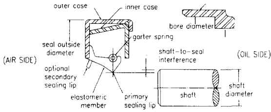
Fig. 1 Typical radial lip seal.
