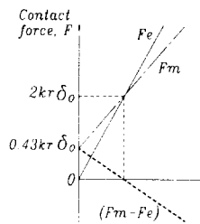
Fig. 6 The exact and the measured contact forces as a function of interference.
