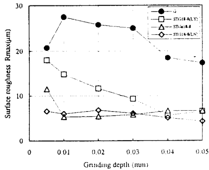
Fig.9 Relationship between surface roughness and grinding depth on Cu
