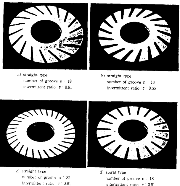
Fig.6 Developed discontinuous grinding wheel with different structure of groove
