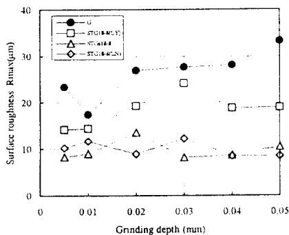
Fig.11 Relationship between surface roughness and grinding depth on Al6061
