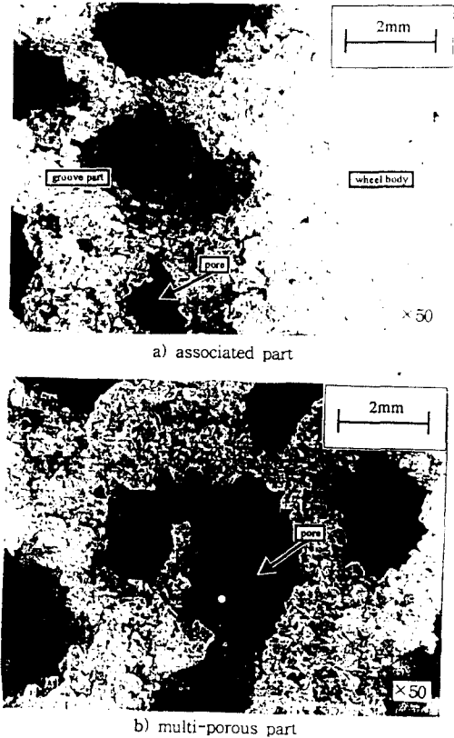
Fig.5 Associated part of the multi-porous grooves with grinding wheel body and porous part
