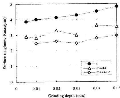
Fig.10 Relationship between surface roughness and grinding depth on Brass
