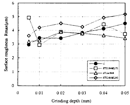
Fig.12 Relationship between surface roughness and grinding depth on SUS304
