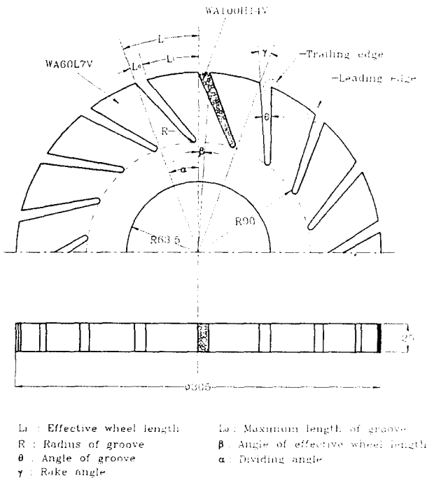
Fig.1 Schematic diagram of the straight type discontinuous grinding wheel(STG) with multi-porous grooves
