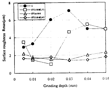
grinding wheel : WA60L7V, workpiece : SM45C grinding speed : 24m/s (1800rpm) table speed : 9.0m/min, feed : 1.25mm/2pass
