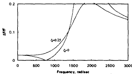
Fig. 15. Theoretical force fluctuation of the normal load with damping ratio. (Applied Load, 49 N; Stiffness, k_2=120000 N/m; Waviness Amplitude, 10 \mu\text{m} )
