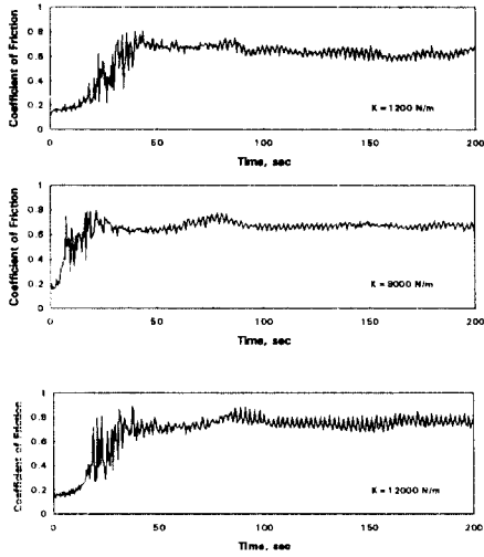
Fig. 3 Coefficient of friction with the different conditions of dynamic stiffness. (Normal load, 49 N; Sliding velocity, 0.1 m/s; Data average duration, 1/3 sec)
