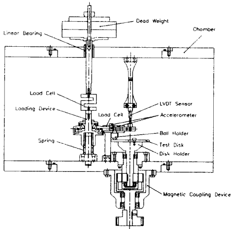
Fig.1 A sectional view of the friction test rig.
