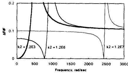
Fig. 13 Theoretical force fluctuation of the normal load with the stiffness. (Applied load, 49 N; Waviness amplitude, 10 \mu\text{m} )
