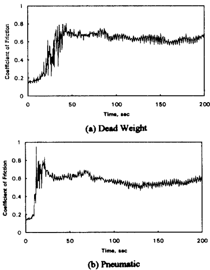
Fig. 4. Coefficients of friction with the different loading methods. (Normal load, 49 N; Sliding velocity, 0.1 m/s; Data average duration, 1/3 sec)
