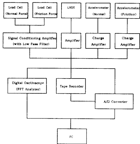
Fig. 2 A block diagram of the measuring system.
