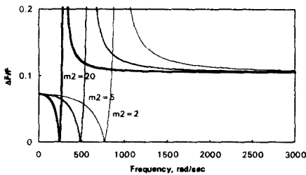
Fig. 14. Theoretical force fluctuation of the normal load with the mass. (Applied load, 49 N; Waviness amplitude, 10 \mu\text{m} )
