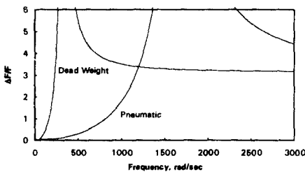
Fig. 16. Theoretical force fluctuation of the normal load with the loading method. (Dead Weight, m_2=5 kg, k_2=1200 N/m; Pneumatic, \zeta=0.1 , k_2=1200 ; Waviness Amplitude, 300 \mu\text{m} )
