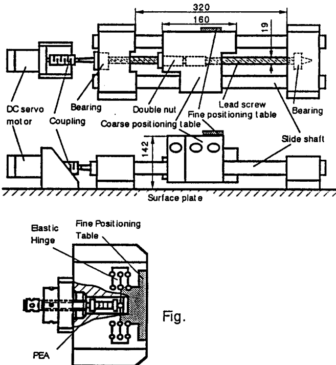
Fig.1 Coarse and Fine Positioning Apparatus
