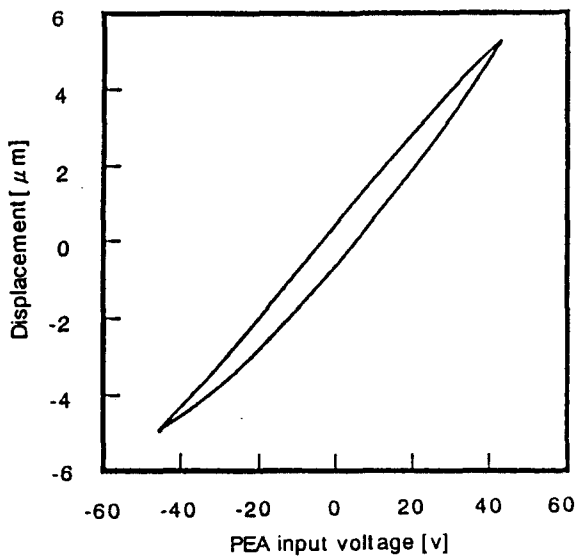
Fig.8 Characteristic of Fine Apparatus (42V)
