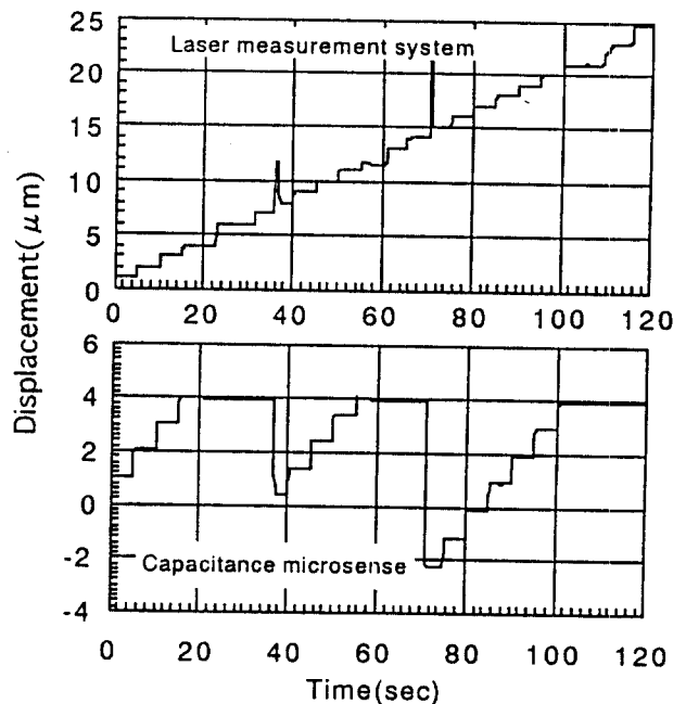
Fig.6 Control of the 1 \mu m Step Positioning
