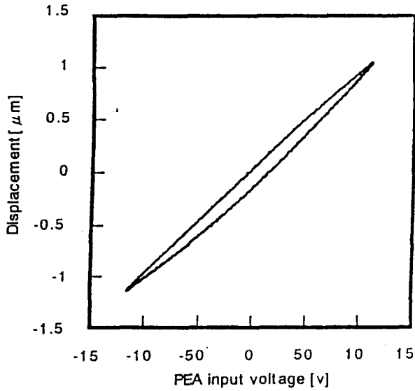
Fig.7 Characteristic of Fine Apparatus (11V)
