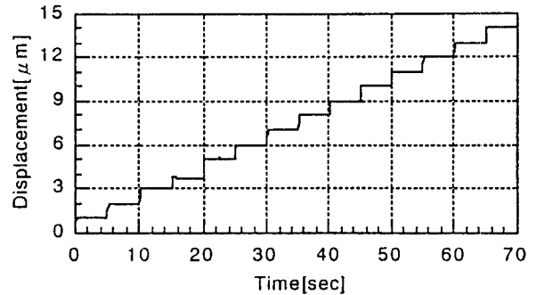
Fig.5 Long Stroke Positioning of 1 \mu m Step for Dual Positioning
