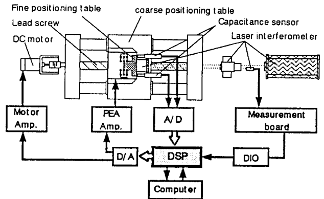
Fig.3 Schematic Diagram of Precision Dual Positioning System
