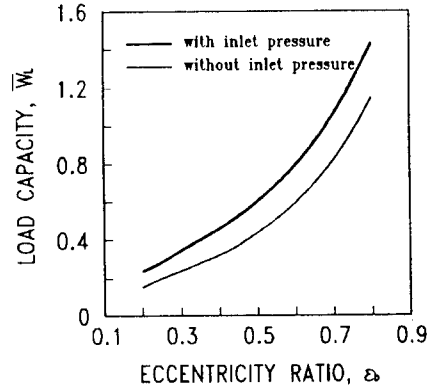
Fig.3 Load capacity vs. eccentricity ratio ( Re=2000 )
