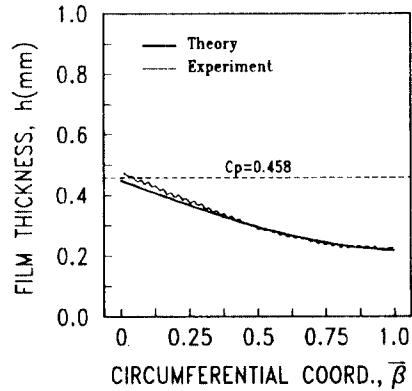
(b) Film thickness
