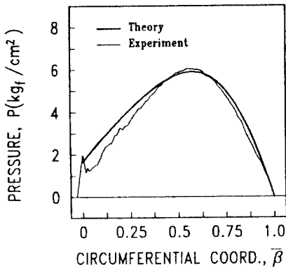
(a) Film Pressure
