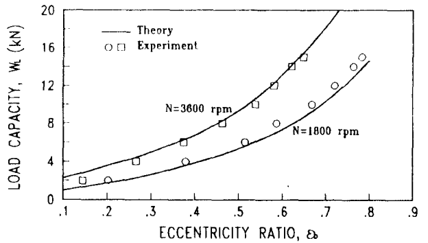
Fig.9 Comparison between theory and experiment of load capacity with eccentricity ratio
