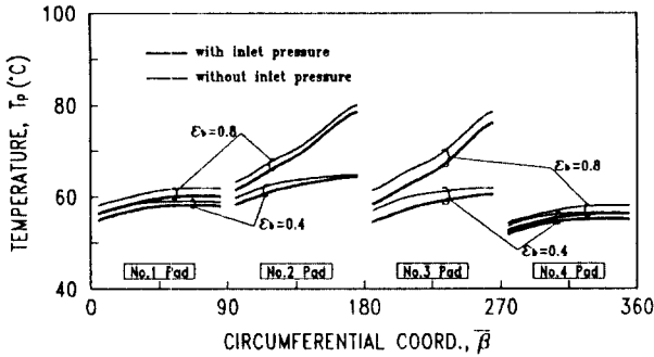
Fig.5 Circumferential distribution of bearing surface temperature in the mid-plane ( Re=2000 )
