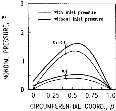
(a) Film Pressure
