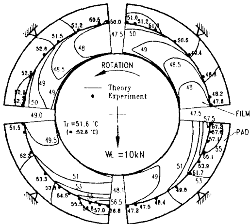
Fig.8 Isotherms in the mid-plane ( N = 3600 rpm, W_L = 10 kN)
