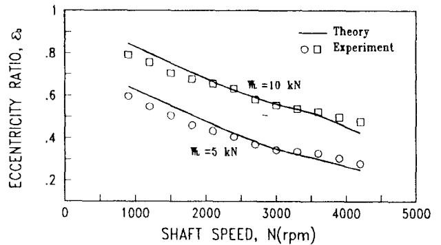
Fig.10 Comparison between theory and experiment of leccentricity ratio with shaft speed
