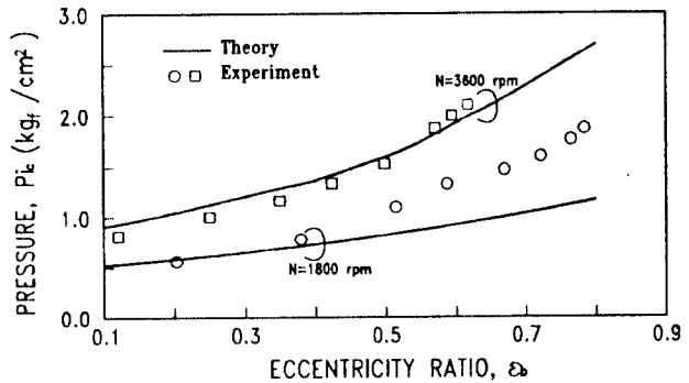
Fig.7 Comparison between theory and experiment of inlet pressure of No.2 pad in the mid-plane
