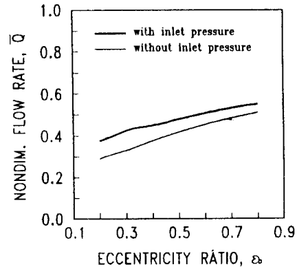
Fig.4 Flow rate vs. eccentricity ratio
