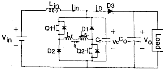
Fig.2 The boost ZVS PWM converter
