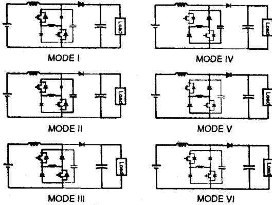
Fig.3 Topological mode diagram
