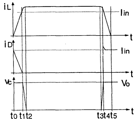
Fig.4 Circuit waveforms
