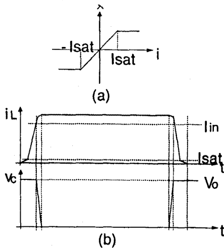
Fig.5 The effect of saturable reactor (a) \lambda - i characteristic curve of L_s , (b) i_L and v_c waveforms
