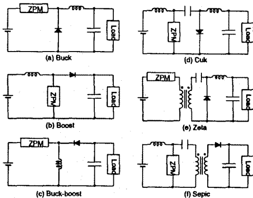
Fig. 6 ZVS PWM converter family
