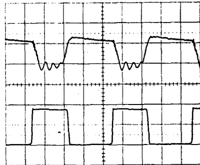
Fig.7 Experimental waveforms of the boost ZVS PWM converter without inserting L_s upper trace : i_L (5A/div) lower trace : v_c (50V/div) time scale : 1 \mu sec/div
