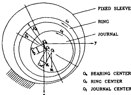
Fig. 1 Circumferentially grooved floating ring journal bearing
