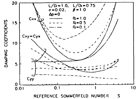
Fig. 10 The effect of supply pressure on damping coefficients
