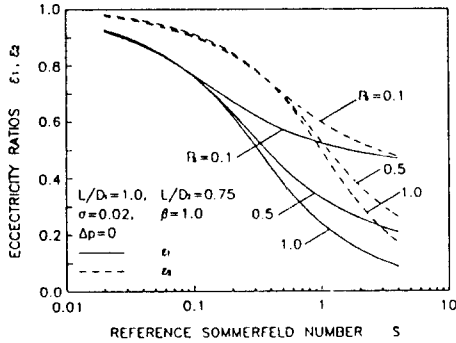
Fig. 2 The effect of supply pressure on eccentricity ratios, \beta=1.0
