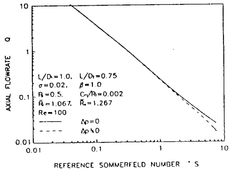
Fig. 15 The effect of pressure drop on axial flowrate
