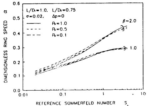
Fig. 6 The effect of supply pressure on dimensionless ring speed
