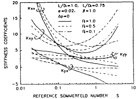
Fig. 9 The effect of supply pressure on stiffness coefficients
