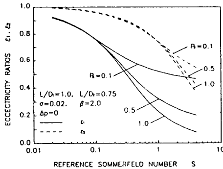
Fig. 3 The effect of supply pressure on eccentricity ratios, \beta=2.0
