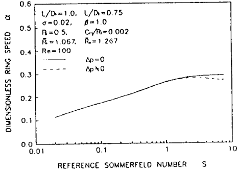
Fig. 13 The effect of pressure drop on dimensionless ring speed
