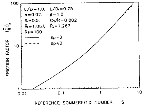
Fig. 14 The effect of pressure drop on friction factor
