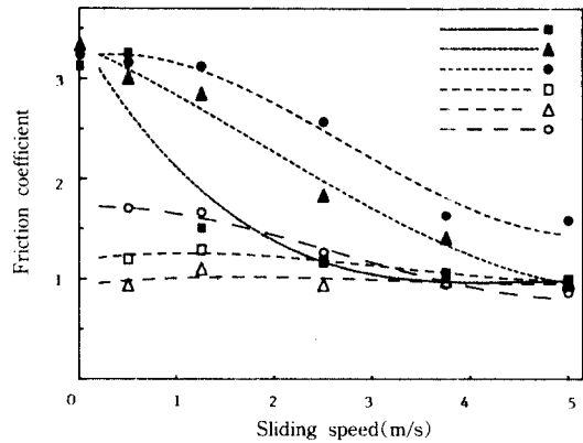
Fig. 4. Friction coefficients of the composite varying with sliding speed for each humidity and fiber orientation.
