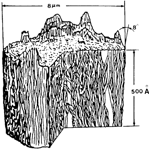
Fig. 6. Schematic three-dimensional structure of carbon fiber.
