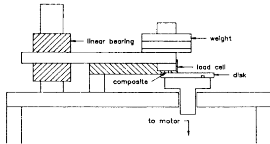
Fig. 2. Schematic diagram of the pin-on-disk set-up used for friction and wear tests in the experiment.
