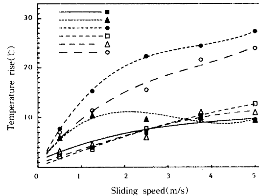
Fig. 5. Temperatures rise 1 mm beneath the center of composite friction surface varying with sliding speed for each humidity and fiber orientation.
