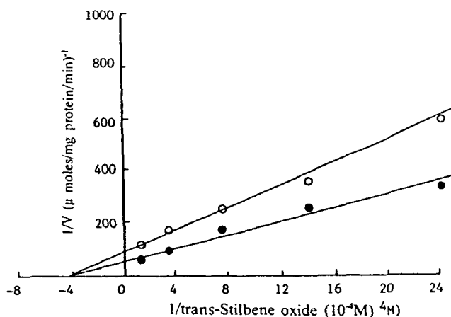
Fig. 1. Double reciprocal plots of the hepatic cytosolic epoxide hydrolase activity in mice for trans-stilbene oxide.
