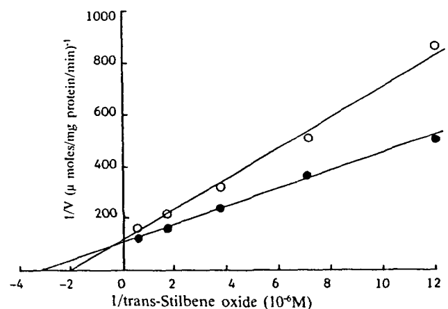
Fig. 3. Double reciprocal plots of the hepatic cytosolic epoxide hydrolase activity for trans-stilbene oxide.
