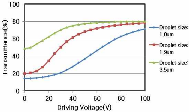
Fig. 6. Electro-optical properties of PDLC cells with single LC droplet sizes of 1.0, 1.9, and 3.5 \mu\text{m} .
