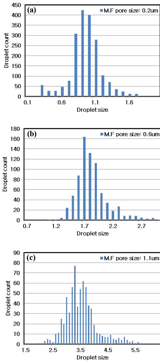
Fig. 5. Liquid crystal droplet size distribution of emulsion made by using membrane filter with pore size of (a) 0.2 \mu\text{m} , (b) 0.6 \mu\text{m} , and (c) 1.1 \mu\text{m} .
