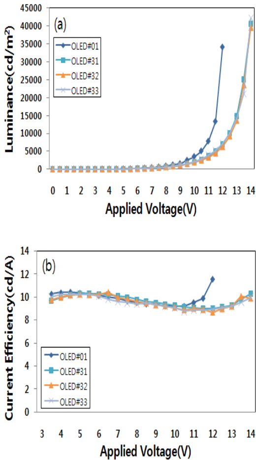
Fig. 5. Emission characteristics of OLEDs with an inorganic protective film between OLED and flat glass cover. (a) luminance-applied voltage, (b) current efficiency-applied voltage.
