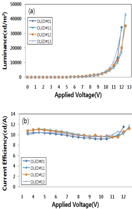
Fig. 3. Emission characteristics of OLEDs with an inorganic protective film without epoxy. (a) luminance-applied voltage, (b) current efficiency-applied voltage.
