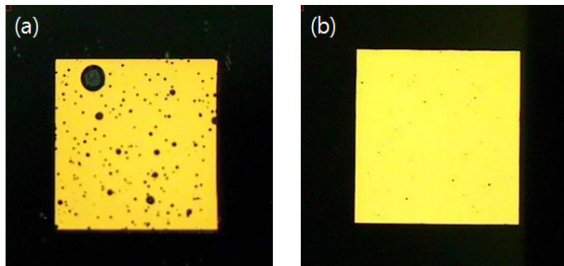
Fig. 7. Picture of OLED with (a) epoxy and (b) LiF/Al/Al/epoxy.
