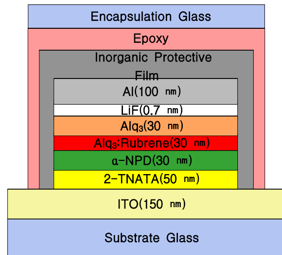
Fig. 1. Encapsulation structure of OLED with an inorganic protective film between OLED and flat glass.
