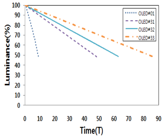
Fig. 6. Lifetime characteristics of OLEDs with an inorganic protective film between OLED and flat glass cover.
