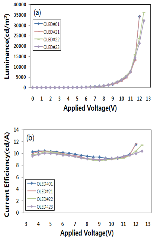
Fig. 4. Emission characteristics of OLEDs with inorganic protective film and epoxy (a) luminance-applied voltage, (b) current efficiency-applied voltage.
