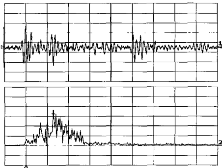
Ch.1 : Acoustic signal [500 mV/div, 50 μs/div] Ch.2 : FFT result [24.5 mV/div, 50 kHz/div] (c) 권선-권선
