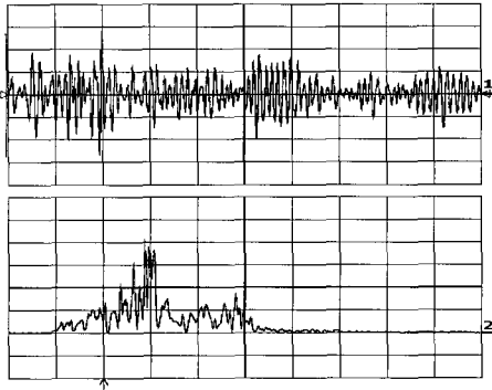
Ch.1 : Acoustic signal [500 mV/div, 50 μs/div] Ch.2 : FFT result [39.5 mV/div, 50 kHz/div] (a) 칩-평판
