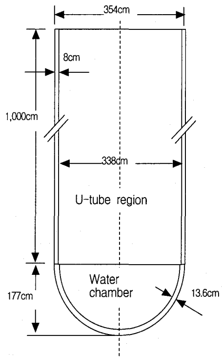
Fig. 1. The geometry of S/G in Kori nuclear power plant unit 1.
