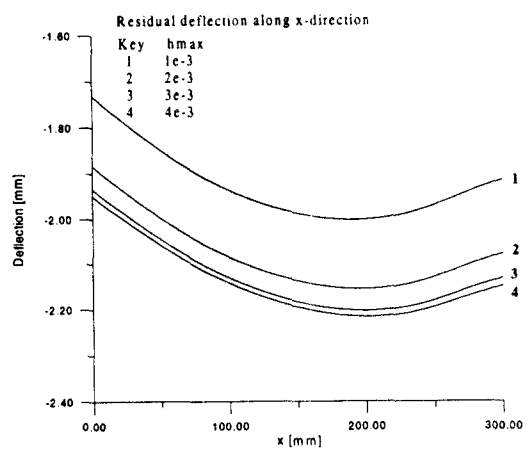
Figure 10(b): Influence on deflection by change in h_{max}
