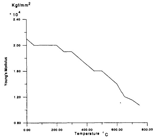
Figure 3(b) Young's modulus
