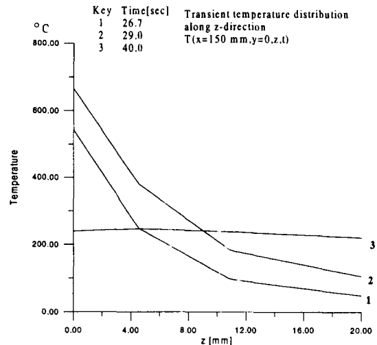
Figure 7(b): Transient temperature distribution along z -direction
