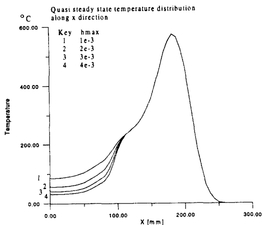
Figure 10(a): Influence on temperature distribution by change in h_{max}
