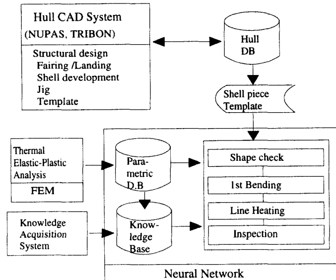
Figure 1: System configuration of plate forming
