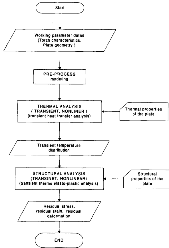
Figure 4: Schematic diagram of the analysis
