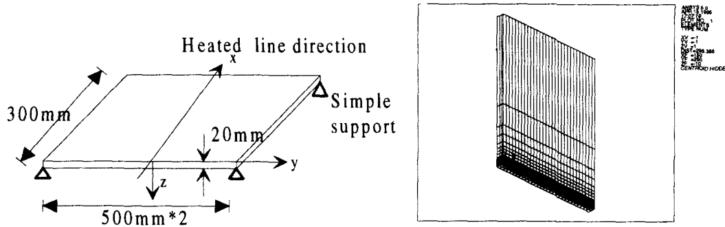
Figure 5: Coordinate system and the finite element analysis model
