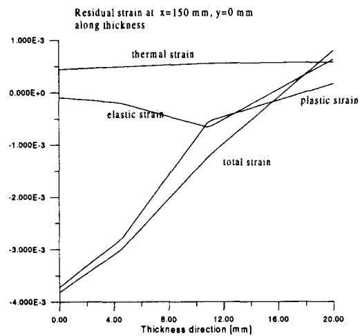
Figure 8(b): Residual strain at mid-plate
