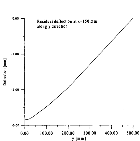
Figure 8(a): Residual deflection along y -direction
