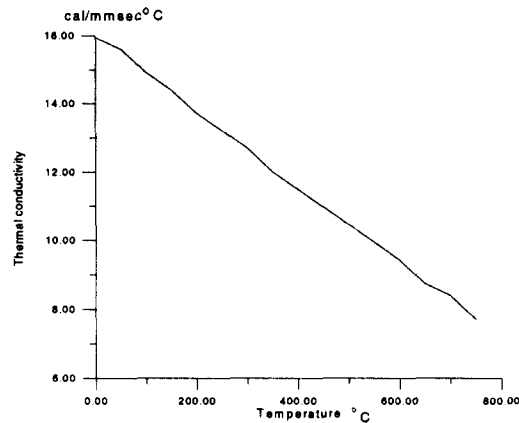
Figure 3(d): Thermal conductivity coefficient
