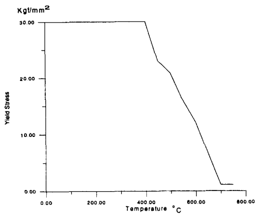
Figure 3(c): Yield stress
