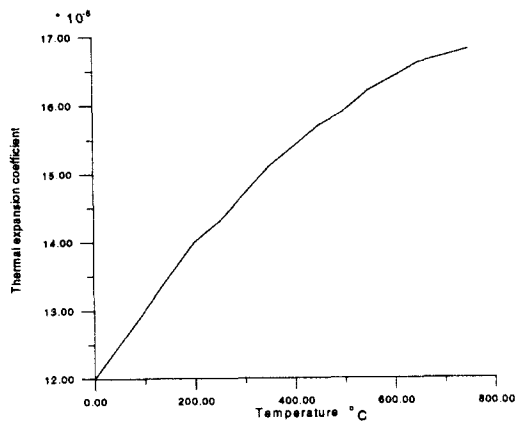
Figure 3(a): Thermal expansion coefficient
