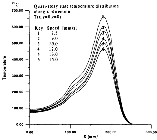
Figure 9(a): Temperature distributions
