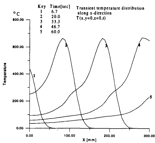
Figure 7(a): Transient temperature distribution along x -direction
