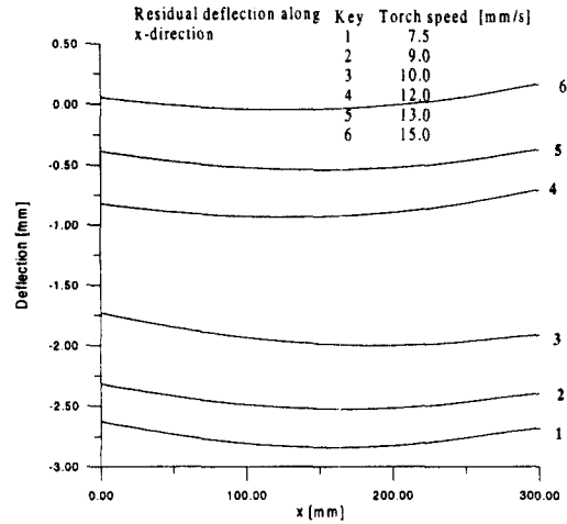
Figure 9(b): Residual deflection along x-direction
