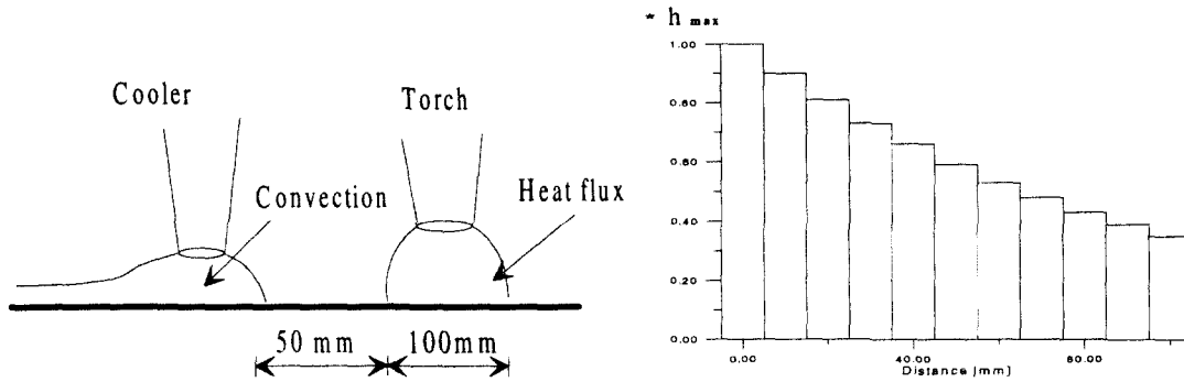
Figure 6: Heat convection coefficient distribution
